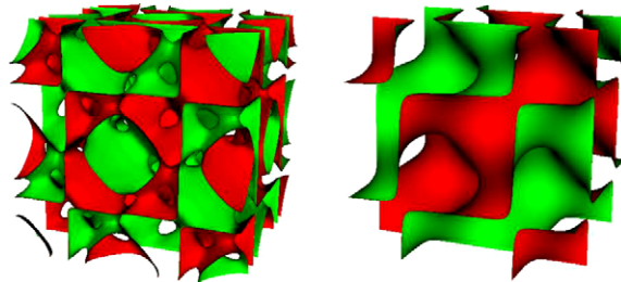
Fig. 9. Evolution of a triply-periodic surface with the symmetry of the Schwartz D surface to the Schwartz D surface (right). The initial structure (left) is obtained by modifying the PNS approximation to the Schwartz D surface so that the second term dominates.
